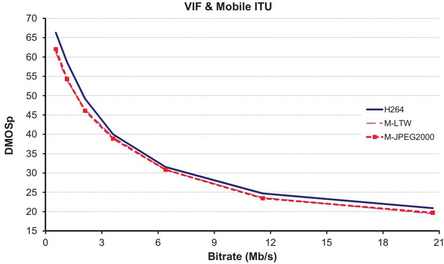
FIG. 8: R/D performance evaluation of the three video codecs using Mobile ITU video sequence by means of VIF metric
